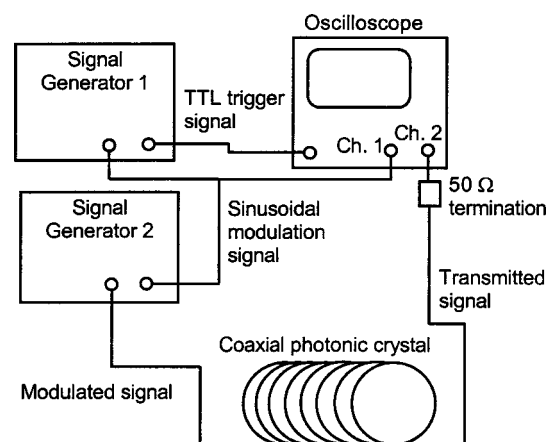
FIG. 1. Experimental arrangement for demonstrating negative group velocity tunneling. The output of signal generator 2 is amplitude modulated by the output of signal generator 1.
